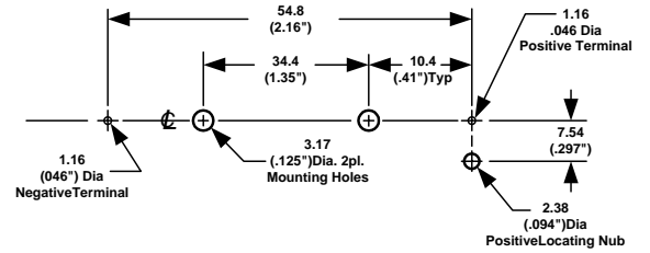
Standard Pc Version P.C. Board Hole layout
