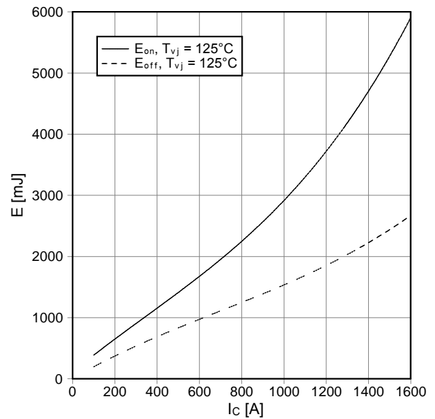
Schaltverluste IGBT-Wechselr. (typisch) switching losses IGBT-inverter (typical) E_{on} = f(I_c) , E_{off} = f(I_c) V_{GE} = \pm 15\text{ V} , R_{Gon} = 2,7\ \Omega , R_{Goff} = 6,8\ \Omega , V_{CE} = 1800\text{ V} , C_{GE} = 220\text{ nF}
