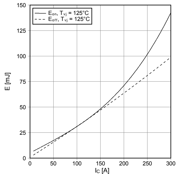
Schaltverluste IGBT-Wechselr. (typisch) switching losses IGBT-inverter (typical) E_{on} = f(I_c) , E_{off} = f(I_c) V_{GE} = \pm 15\text{ V} , R_{Gon} = 9.1\ \Omega , R_{Goff} = 9.1\ \Omega , V_{CE} = 900\text{ V}
