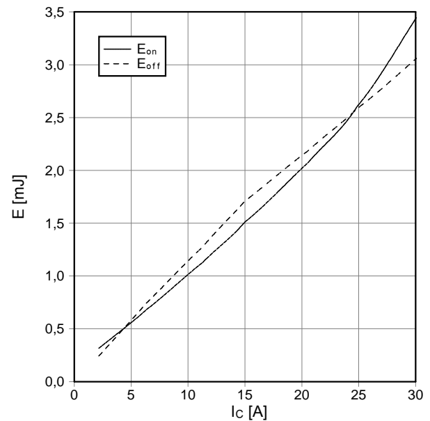
Schaltverluste IGBT-Wechselr. (typisch) switching losses IGBT-inverter (typical) E_{on} = f(I_c) , E_{off} = f(I_c) V_{GE} = \pm 15\text{ V} , R_{Gon} = 62\ \Omega , R_{Goff} = 62\ \Omega , V_{CE} = 600\text{ V} , T_{vj} = 125^\circ\text{C}
