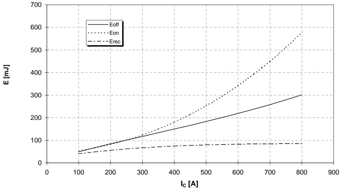
Schaltverluste (typisch) E_{on} = f(I_C) , E_{off} = f(I_C) , E_{rec} = f(I_C) Switching losses (typical) R_{gon} = 2,7\Omega ; R_{goff} = 3,6\Omega , V_{CE} = 900V , T_j = 125^\circ C
