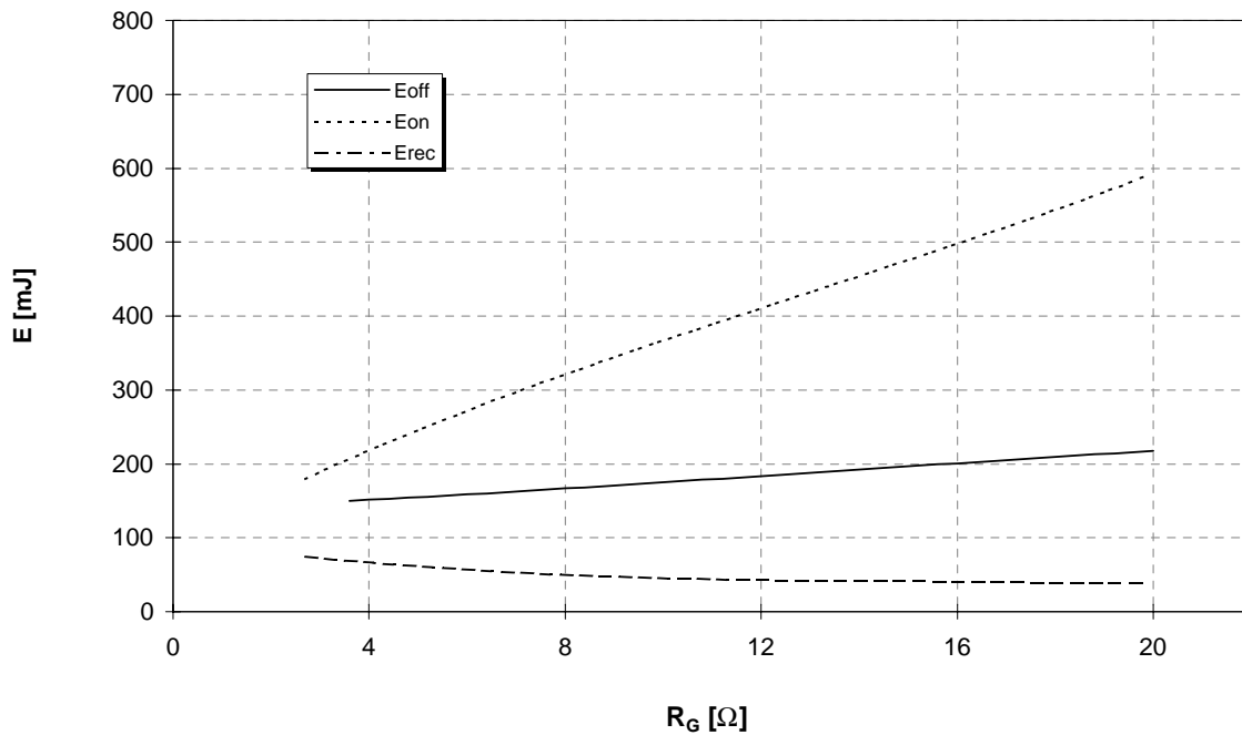
Schaltverluste (typisch) E_{on} = f(R_G) , E_{off} = f(R_G) , E_{rec} = f(R_G) Switching losses (typical) I_C = 400A , V_{CE} = 900V , T_j = 125^\circ C
