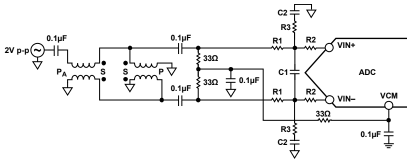
Figure 30. Differential Double Balun Input Configuration
