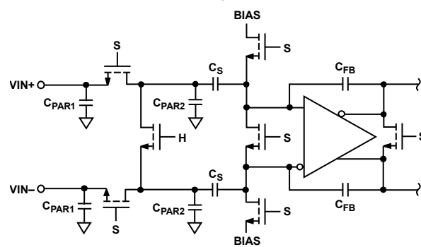
Figure 26. Switched-Capacitor Input
