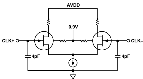
Figure 31. Simplified Equivalent Clock Input Circuit
