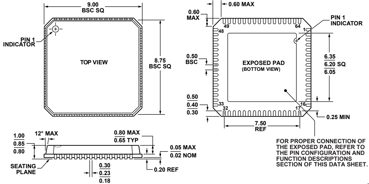
Figure 47. 64-Lead Lead Frame Chip Scale Package [LFCSP_VQ] 9 mm × 9 mm Body, Very Thin Quad (CP-64-4) Dimensions shown in millimeters
