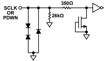
Figure 23. Equivalent SCLK or PDWN Input Circuit
