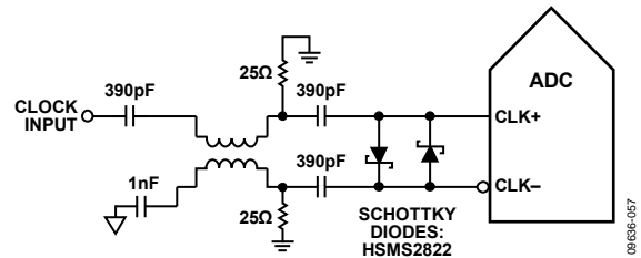
Figure 53. Balun-Coupled Differential Clock (Up to 625 MHz)
