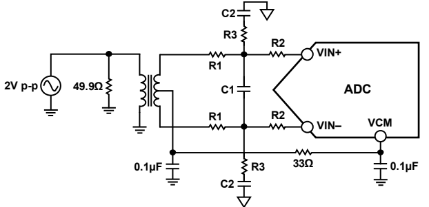
Figure 29. Differential Transformer-Coupled Configuration
