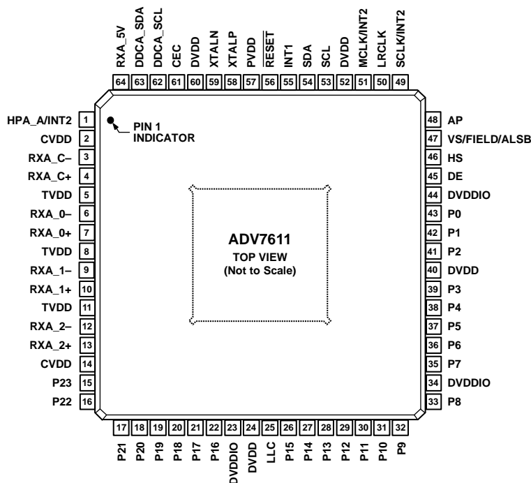
Figure 7. Pin Configuration
