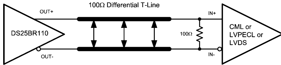
Typical DS25BR110 Output DC-Coupled Interface to an LVDS, CML or LVPECL Receiver
