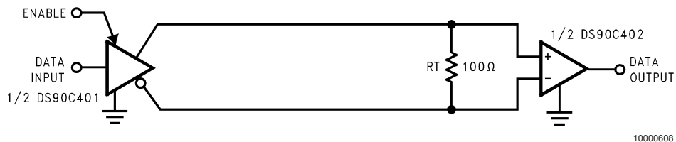
FIGURE 3. Point-to-Point Application
