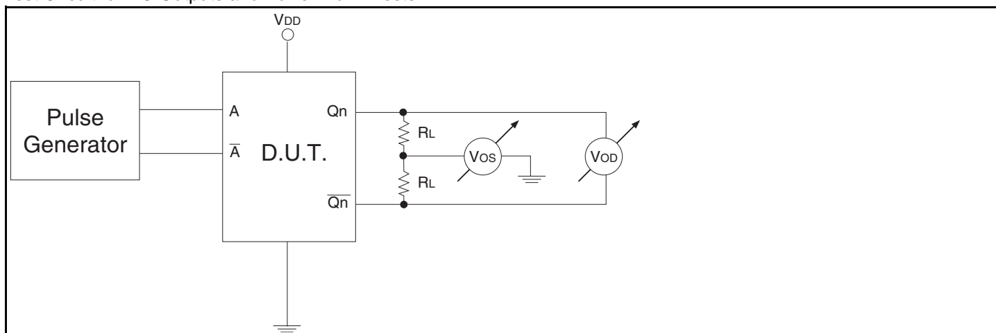
Test Circuit for DC Outputs and Power Down Tests
