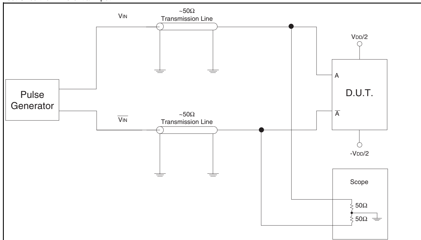
Test Circuit for Differential Input
