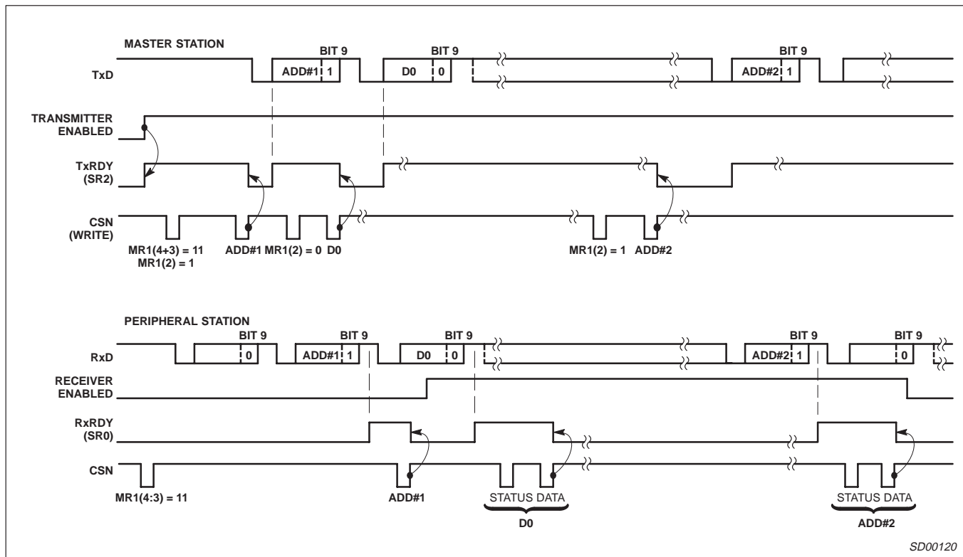
Figure 14. Wake-Up Mode
