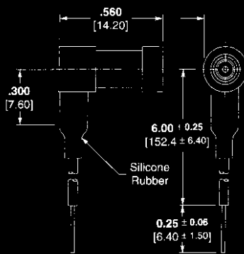
Receptacle (Right-Angle) Part Number 448659-1
