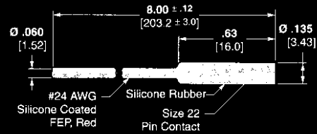
Receptacle Part Number 443958-1
