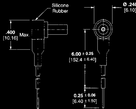
Plug (Right-Angle) Part Number 448661-1
