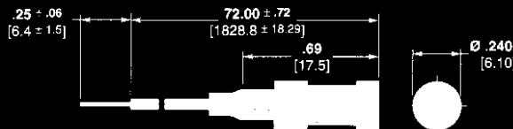
Receptacle Part Number 448658-1
