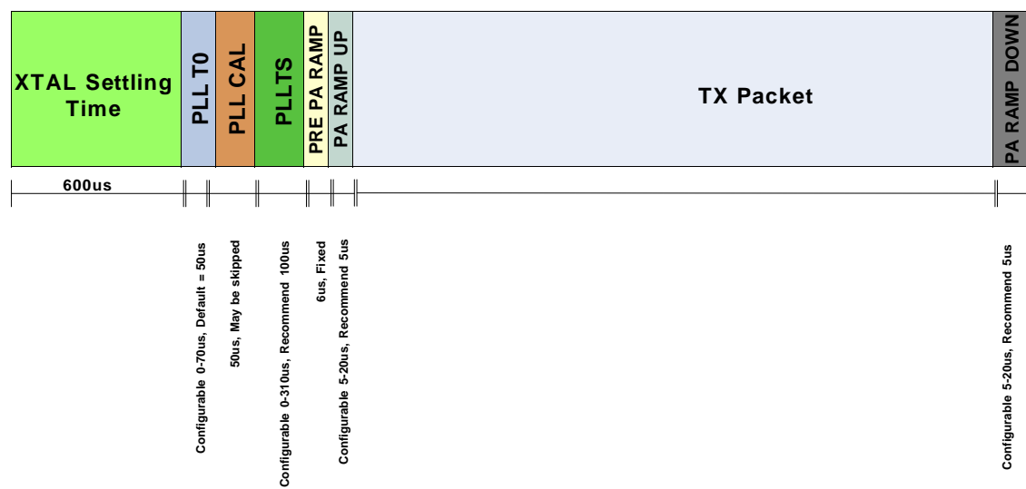
Figure 8. TX Timing
