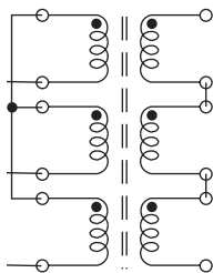
Figure 5 Turns Ratio: 1:3 or 3:1
