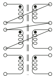
Figure 7 Turns Ratio: 4:1:1
