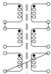
Figure 2 Turns Ratio: 1:1:1
