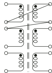
Figure 8 Turns Ratio: 3:1:1:1
