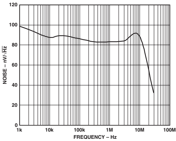
TPC 50. VREF Output Noise Spectral Density vs. Frequency
