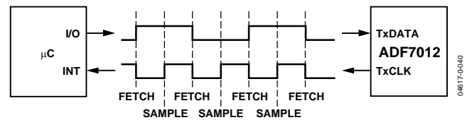
Figure 31. TxCLK/TxDATA Synchronization.
