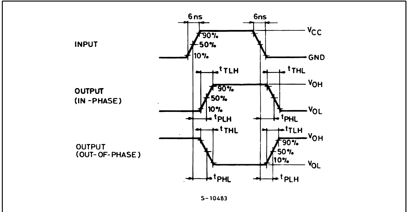
Figure 5: Waveform - Propagation Delay Time (f=1MHz; 50% duty cycle)
