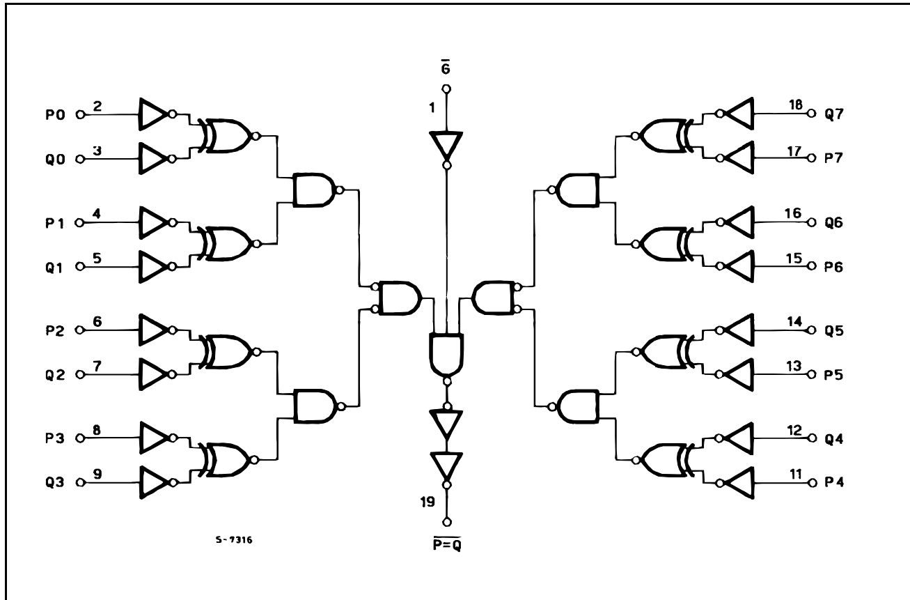
Figure 3: Logic Diagram
