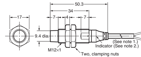
E2A-M12KN08-WP-□□
