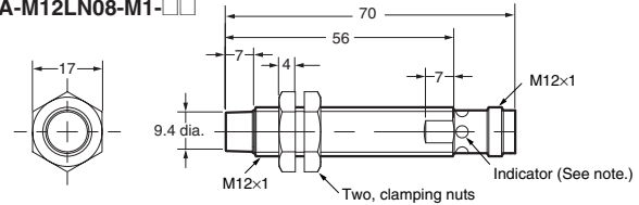
E2A-M12LN08-M1-□□
