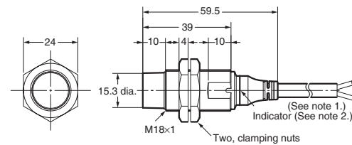
E2A-M18KN16-WP-□□
