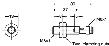
E2A-S08KS02-M5-□□
