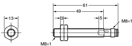
E2A-S08LS02-M5-□□
