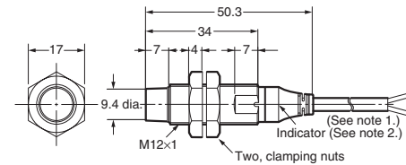
E2A-M12KN08-WP-□□
