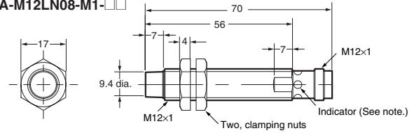
E2A-M12LN08-M1-□□
