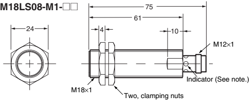
E2A-M18LS08-M1-□□
