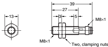
E2A-S08KS02-M5-□□
