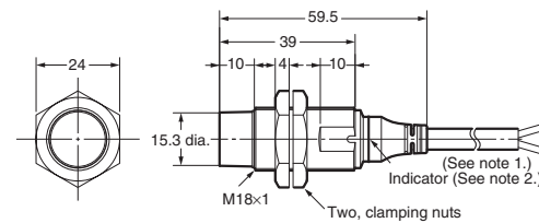
E2A-M18KN16-WP-□□
