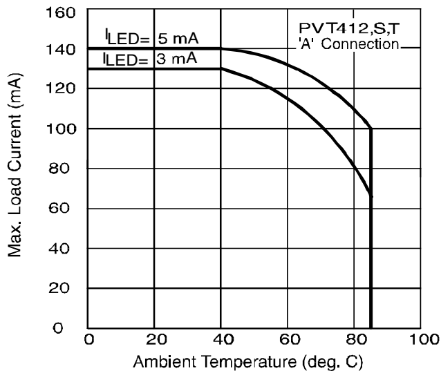
Figure 1. Current Derating Curves*
