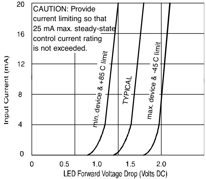
Figure 6. Input Characteristics (Current Controlled)
