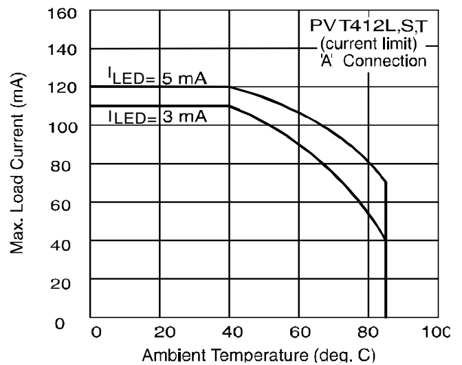
Figure 2. Current Derating Curves*
