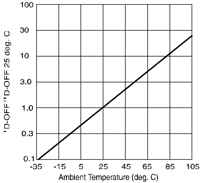
Figure 5. Typical Normalized Off-State Leakage
