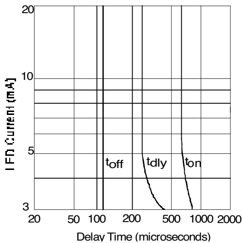
Figure 7. Typical Delay Time
