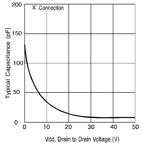
Figure 9. Typical Output Capacitance
