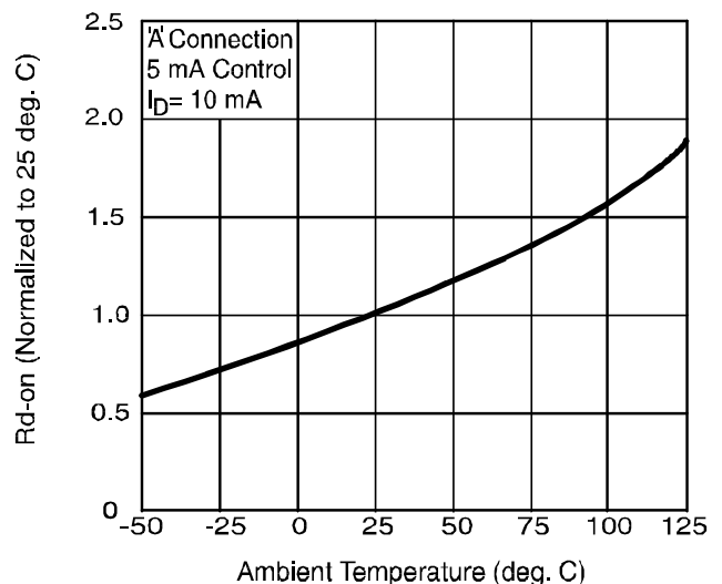
Figure 4. Typical Normalized On-Resistance
