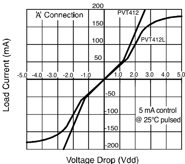
Figure 3. Linearity Characteristics
