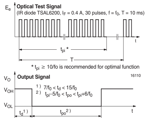
Figure 1. Output Function
