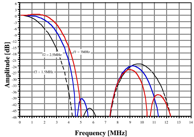
Fig. 13 Chroma Filtering
