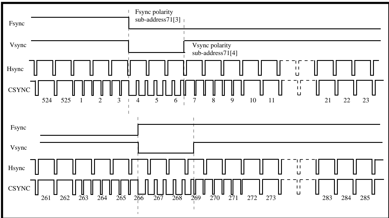
Fig 5 : Sync Timing::525/60 Interlaced System in Master Mode
