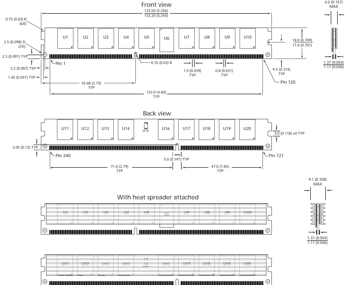
Figure 5: 240-Pin DDR3 RDIMM
