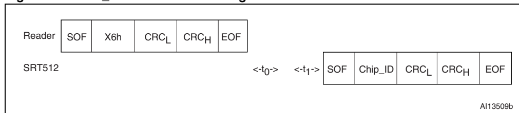
Figure 30. Slot_marker frame exchange between reader and SRT512
