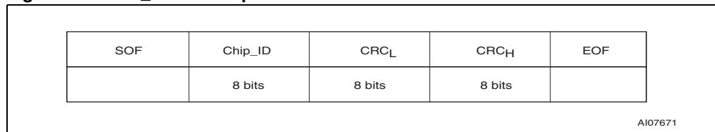
Figure 29. Slot_marker response format
