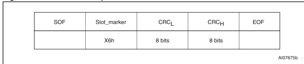
Figure 28. Slot_marker request format
