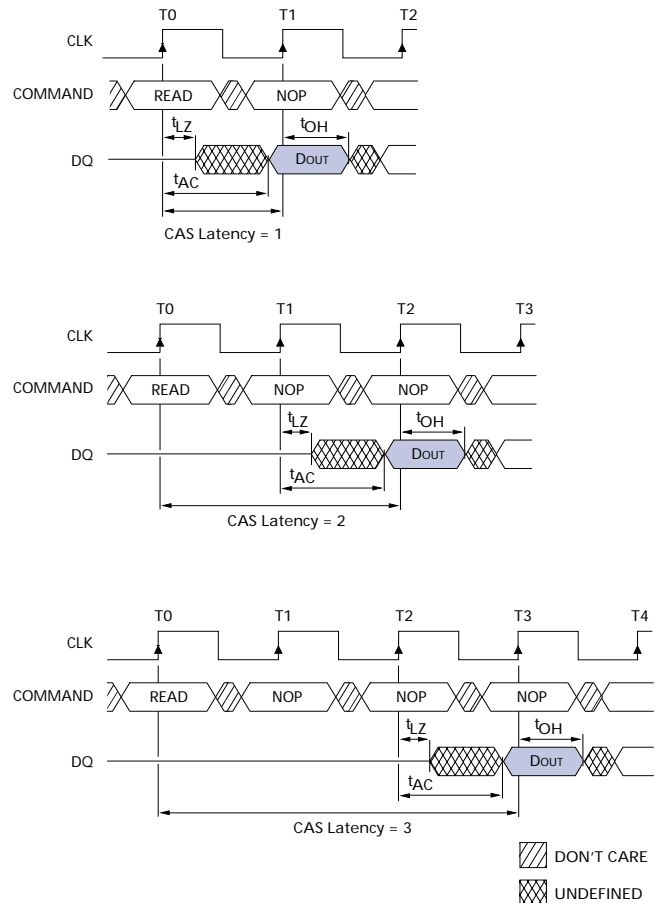
Figure 4: CAS Latency
