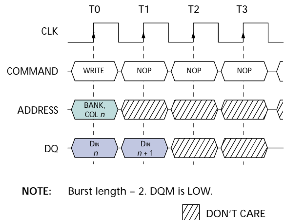
Figure 17: WRITE Burst
