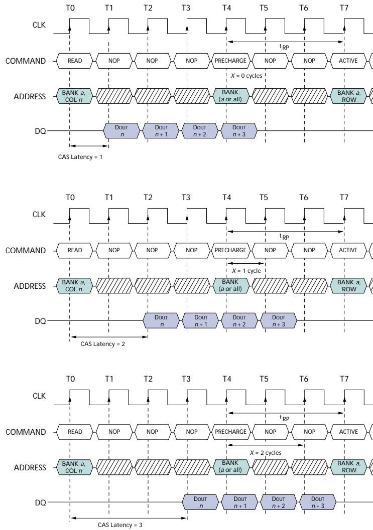
Figure 14: READ to PRECHARGE
