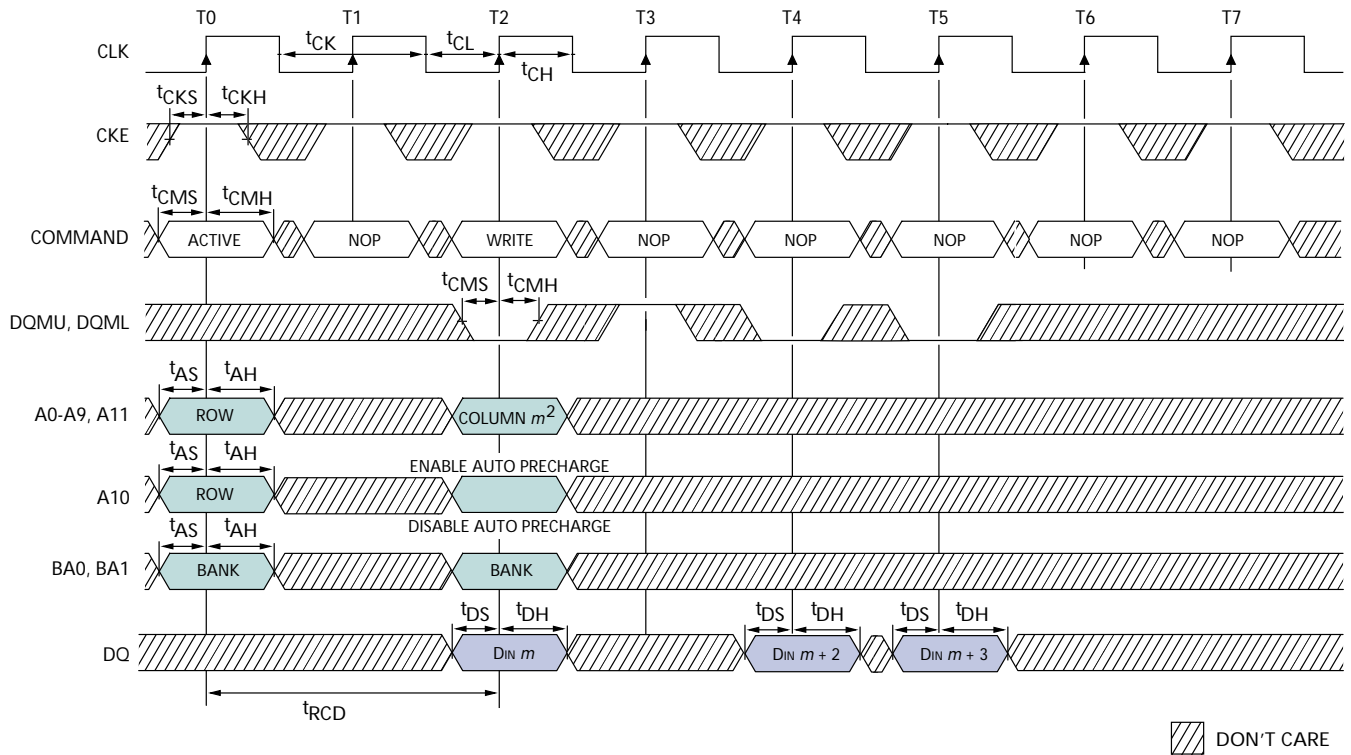
Figure 49: Write - DQM Operation 1
