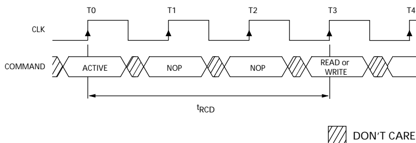
Figure 7: Example: Meeting t_{\text{RCD}} (MIN) When 2 < t_{\text{RCD}}(\text{MIN})/t_{\text{CK}} \leq 3
