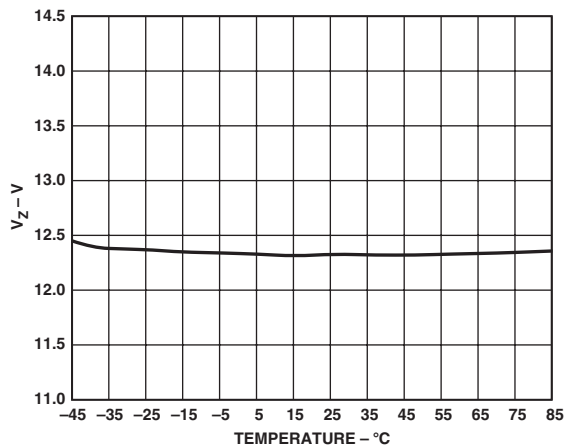
TPC 4. V_Z vs. Temperature
