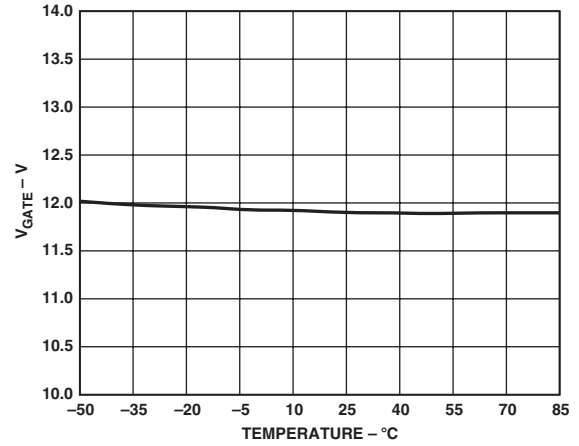
TPC 11. V_{GATE} vs. Temperature
