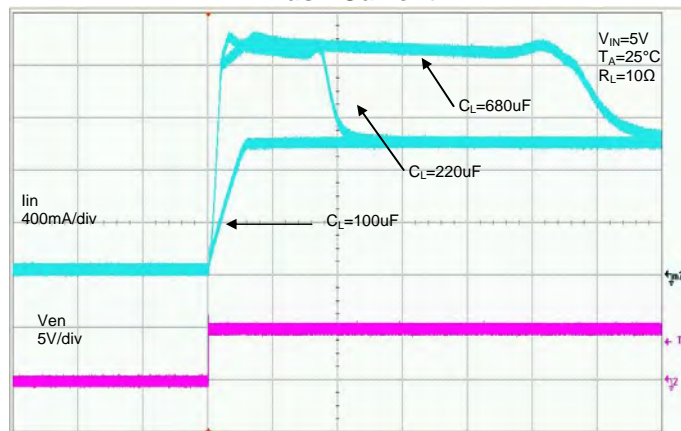
Inrush Current
