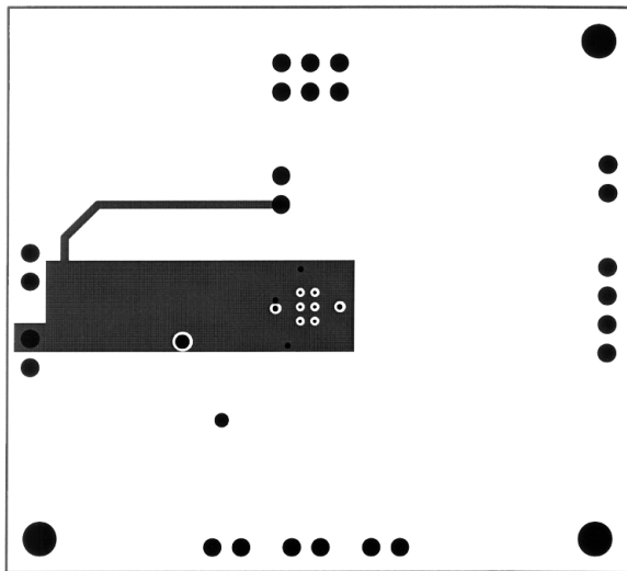
FIGURE 9. Recommended LD PC Board Layout: Inner Layer 1 200395E7
