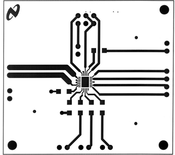
FIGURE 8. Recommended LD PC Board Layout: Top Layer 200395E6
