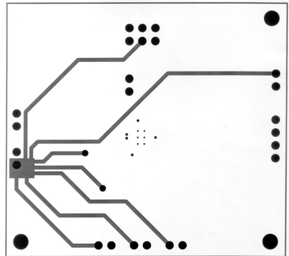
FIGURE 10. Recommended LD PC Board Layout: Inner Layer 2 200395E8
