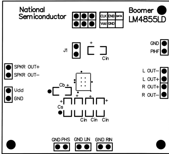
FIGURE 7. Recommended LD PC Board Layout: Top Silkscreen Layer 200395E5
