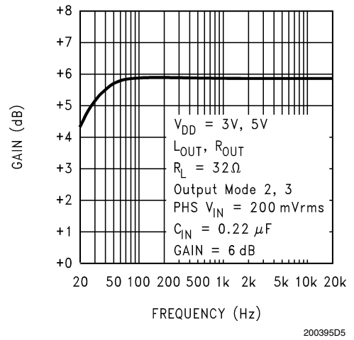
Frequency Response
