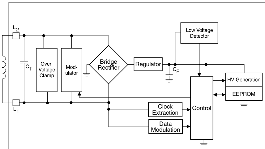
Figure 2. Typical Operating Configuration
