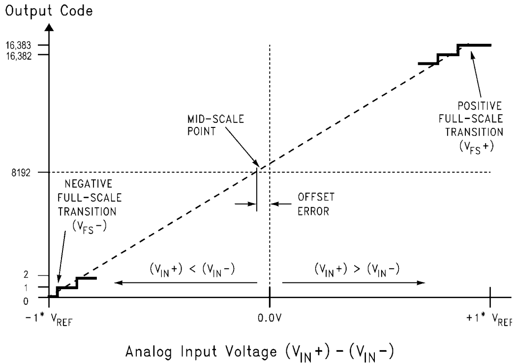
FIGURE 1. Transfer Characteristic (Offset Binary Format)
