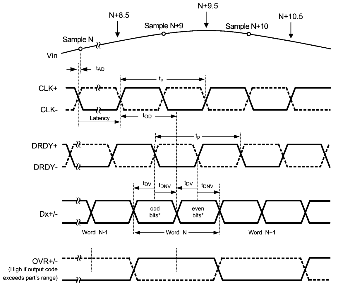
Output Timing
