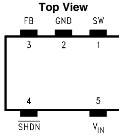
20059111 5-Lead SOT-23 Package See NS Package Number MF05A
