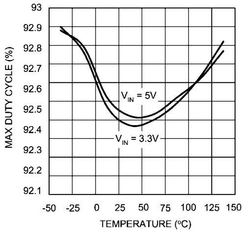
Max. Duty Cycle vs Temperature - "X"
