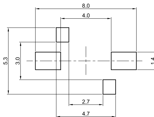
PRINTED CIRCUIT BOARD DIMENSIONS (WHEN VIEWED FROM SWITCH MOUNTING FACE)
