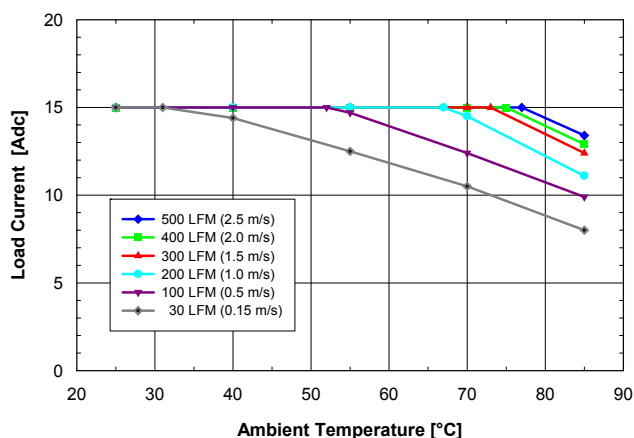
Fig. 3.3V.2: Available load current vs. ambient air temperature and airflow rates for SQ48T15033 converter with D height pins mounted horizontally with V_{in} = 48\text{ V} , air flowing from pin 3 to pin 1, and maximum FET temperature \leq 120\text{ }^\circ\text{C} .
