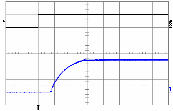
Fig. 2.5V.10: Turn-on transient at full rated load current (resistive) plus 10,000 µF at V_{in} = 48\text{ V} , triggered via ON/OFF pin. Top trace: ON/OFF signal (5 V/div.). Bottom trace: output voltage (1 V/div.). Time scale: 2 ms/div.
