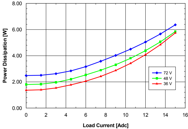
Fig. 2.5V.7: Power dissipation vs. load current and input voltage for SQ48T/S15025 converter mounted vertically with air flowing from pin 3 to pin 1 at a rate of 300 LFM (1.5 m/s) and T_a = 25\text{ }^\circ\text{C} .
