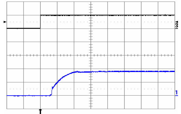
Fig. 1.8V.10: Turn-on transient at full rated load current (resistive) plus 10,000 µF at V_{in} = 48\text{ V} , triggered via ON/OFF pin. Top trace: ON/OFF signal (5 V/div.). Bottom trace: output voltage (1 V/div.). Time scale: 2 ms/div.
