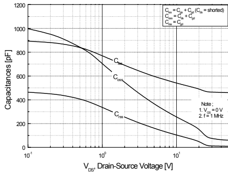
Figure 5. Capacitance Characteristics
