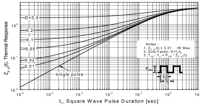
Figure 11-2. Transient Thermal Response Curve for FQPF6N40CF
