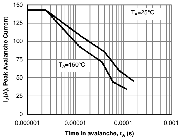
Figure 10: Single Pulse Avalanche capability
