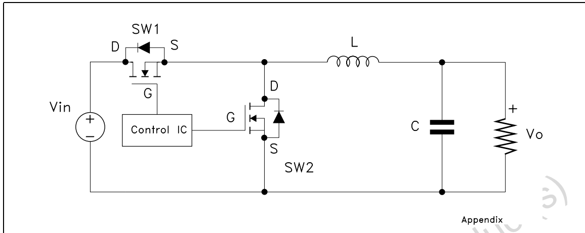
Figure 19. Buck converter
