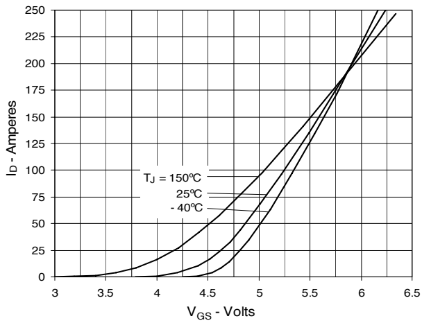
Fig. 7. Input Admittance
