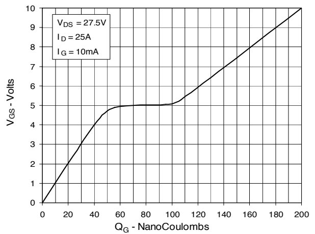
Fig. 10. Gate Charge
