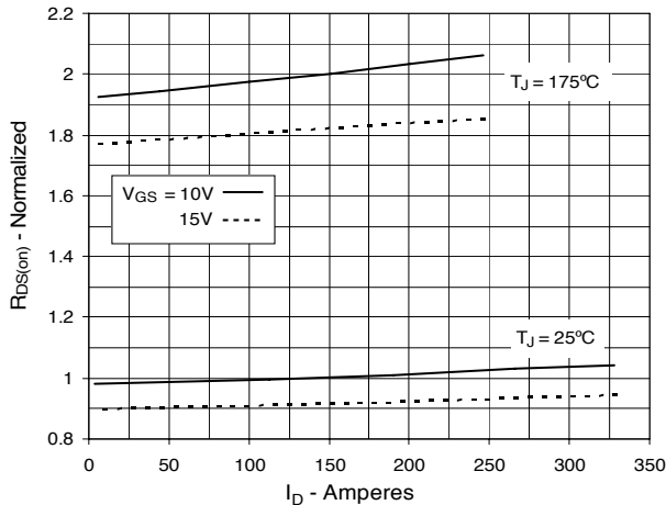
Fig. 5. R_{DS(on)} Normalized to I_D = 140A Value vs. Drain Current
