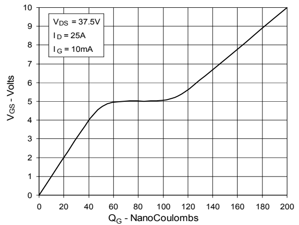
Fig. 10. Gate Charge
