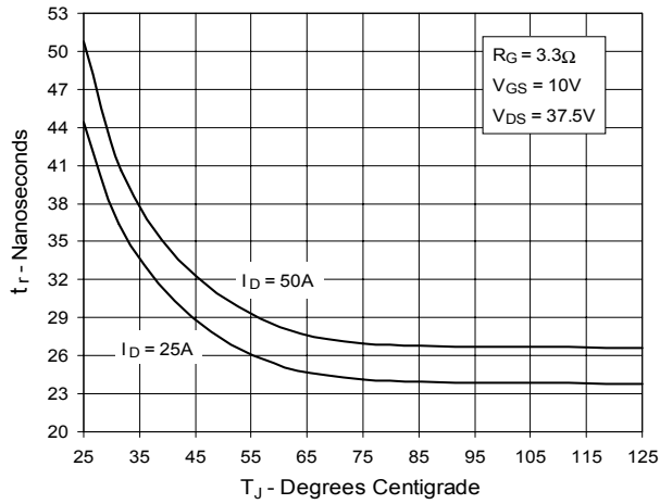
Fig. 13. Resistive Turn-on Rise Time vs. Junction Temperature
