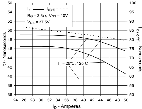
Fig. 17. Resistive Turn-off Switching Times vs. Drain Current
