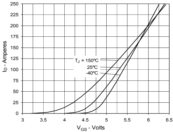
Fig. 7. Input Admittance
