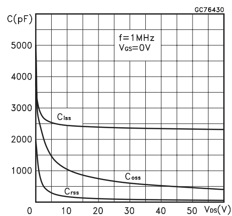
Figure 10. Capacitance Variations
