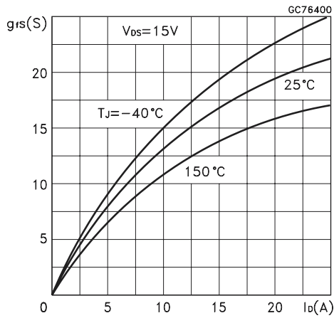
Figure 7. Transconductance
