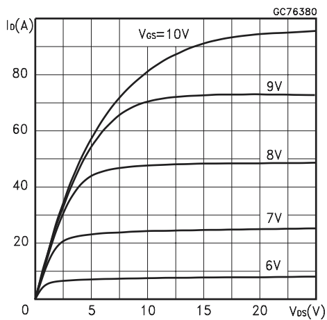
Figure 5. Output Characteristics
