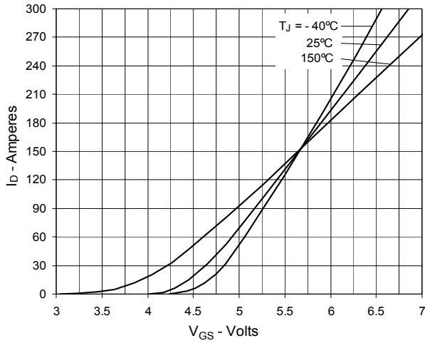
Fig. 7. Input Admittance
