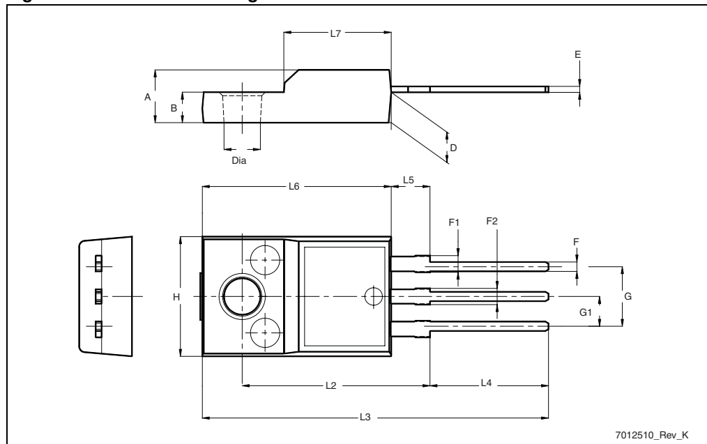
Figure 24. TO-220FP drawing
