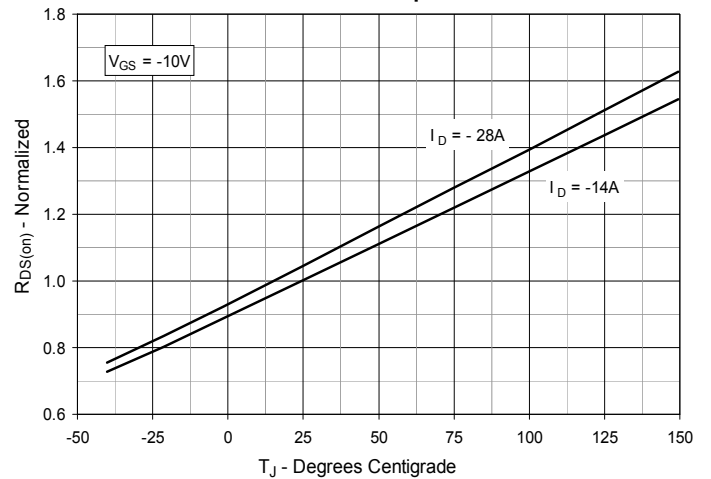
Fig. 4. R_{DS(on)} Normalized to I_D = -14\text{A} vs. Junction Temperature
