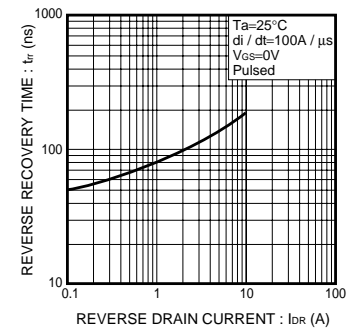
Fig.12 Reverse Recovery Time vs. Reverse Drain Current
