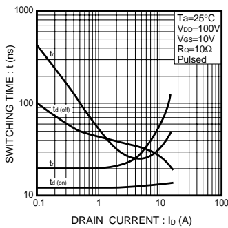
Fig.13 Switching Characteristics
