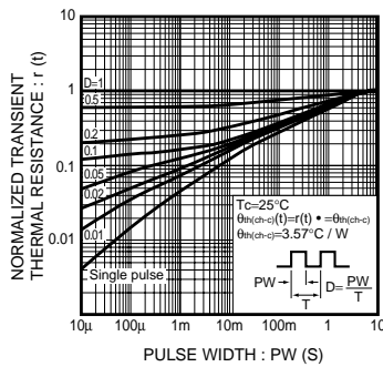
Fig.14 Normalized Transient Thermal Resistance vs. Pulse Width
