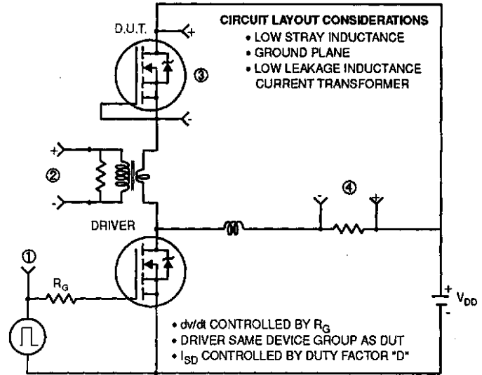
Fig 14. Peak Diode Recovery dv/dt Test Circuit
