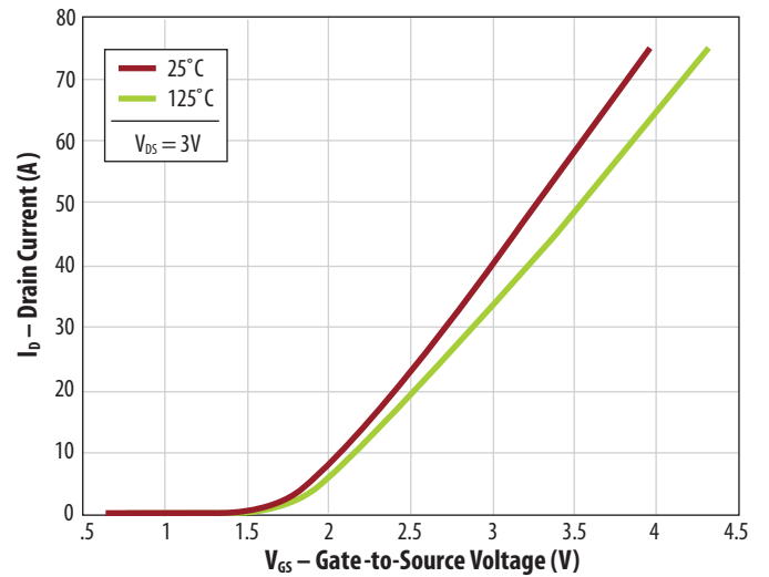
Figure 2: Transfer Characteristics
