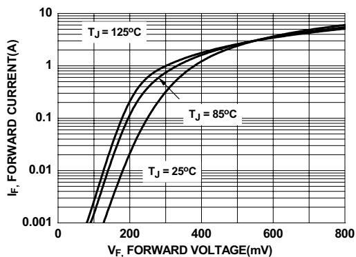
Figure 11. Schottky Diode Forward Voltage
