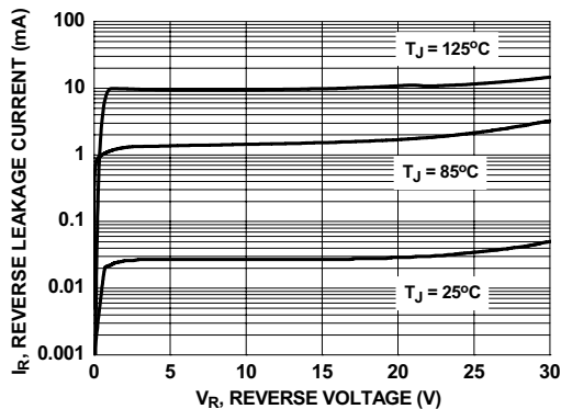
Figure 12. Schottky Diode Reverse Current
