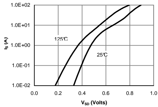
Figure 6: Body-Diode Characteristics (Note E)
