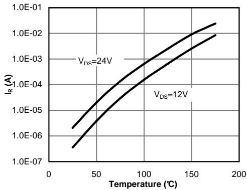
Figure 13: Diode Reverse Leakage Current vs. Junction Temperature
