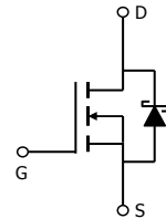
SRFET™ Soft Recovery MOSFET: Integrated Schottky Diode
