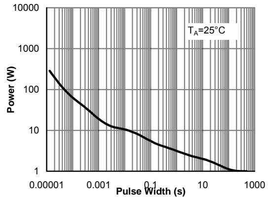
Figure 11: Single Pulse Power Rating Junction-to-Ambient (Note F)
